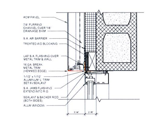
C4 EXT. WINDOW JAMB @ W5 3/4\"/>
