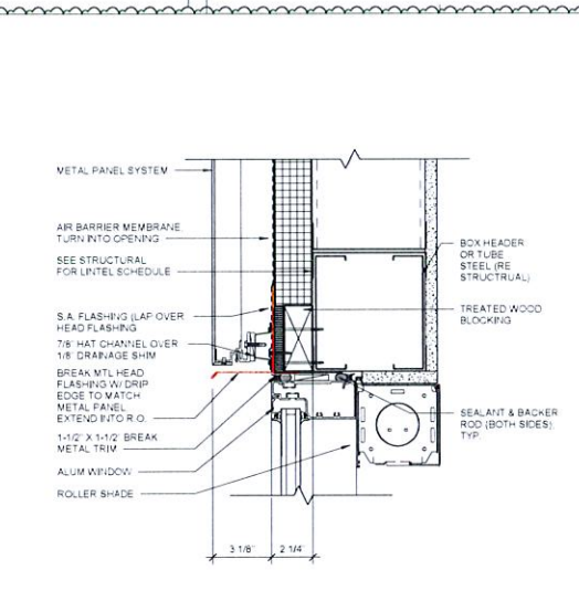
D3 EXT. WINDOW HEAD @ W2 3/4\"/>
