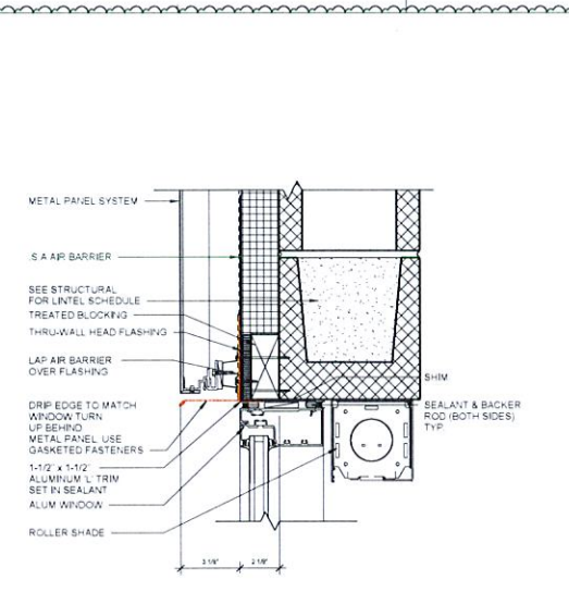
D4 EXT. WINDOW HEAD @ W5 3/4\"/>
