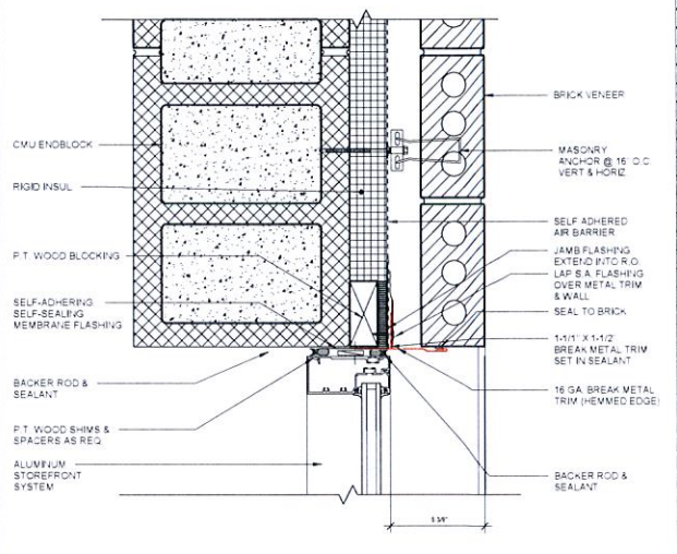
C5 EXT. WINDOW JAMB @ W9 3/4\"/>
