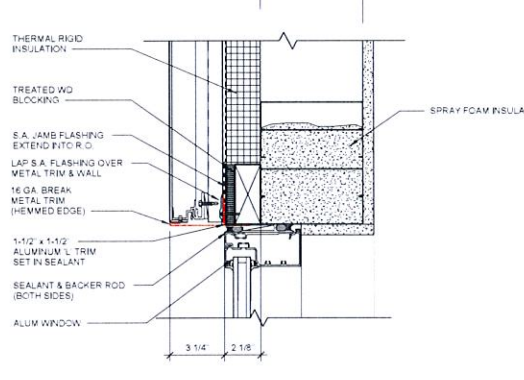
C3 EXT. WINDOW JAMB @ W2 3/4\"/>
