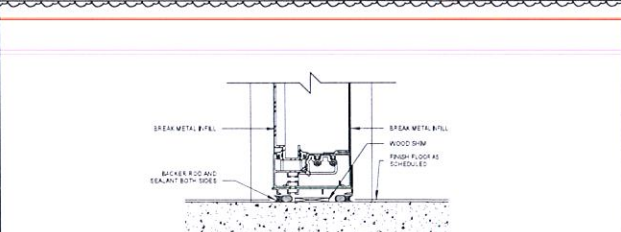
A5 ALUM. FRAME - INTERIOR SILL 3/4\"/>
