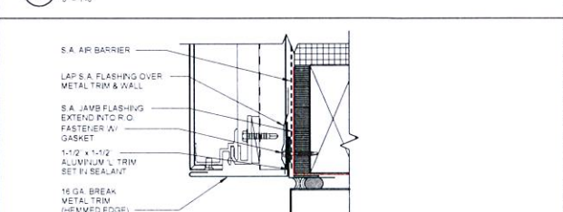
B5 ENLARGED JAMB FLASHING DETAIL 6\"/>
