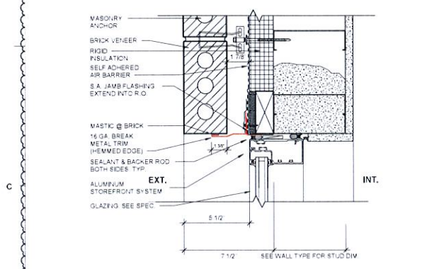
C1 EXT. WINDOW JAMB @ W1 3/4\"/>
