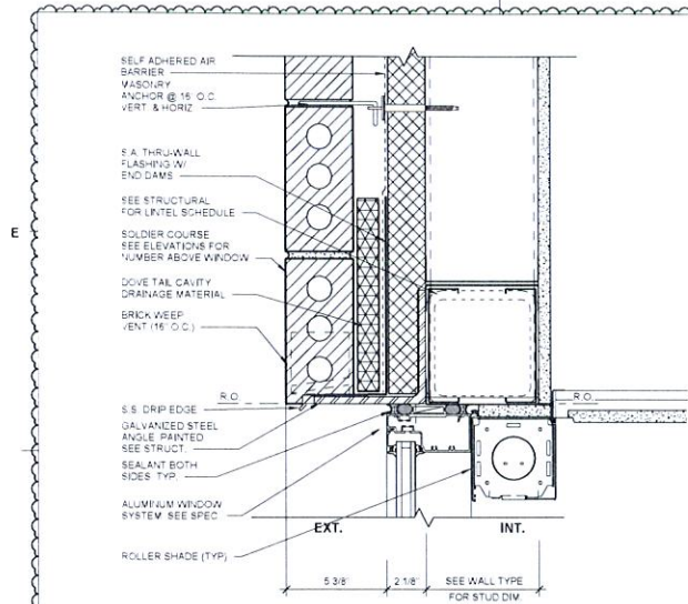
D1 EXT WINDOW HEAD @ W1 3/4\"/>
