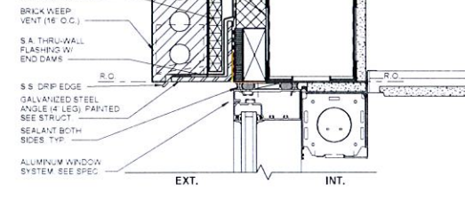
B4 EXT WINDOW HEAD @ W1 (LOOSE LINTEL) 3/4\"/>
