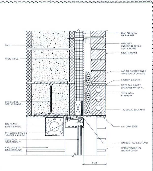
D5 EXT. WINDOW HEAD @ W9 3/4\"/>
