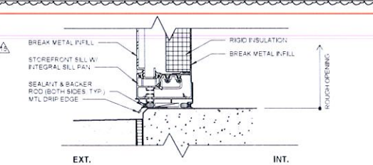
A4 EXT ALUMN. S.F. WINDOW- SILL DETAIL @ SF BASE 3/4\"/>
