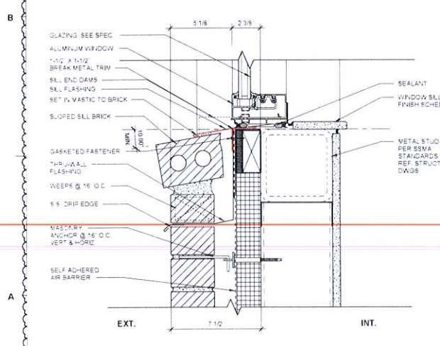
A1 EXT. WINDOW SILL @ W1 3/4\"/>
