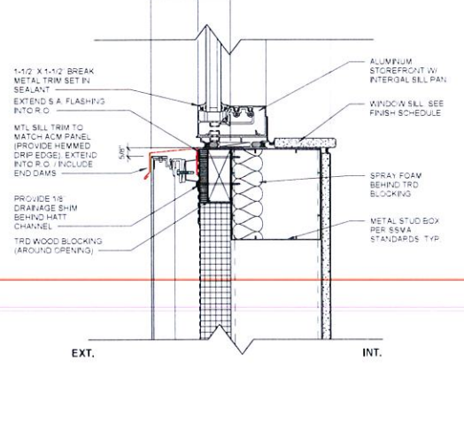
A3 EXT ALUMN. S.F. WINDOW- SILL DETAIL @ W2 3/4\"/>
