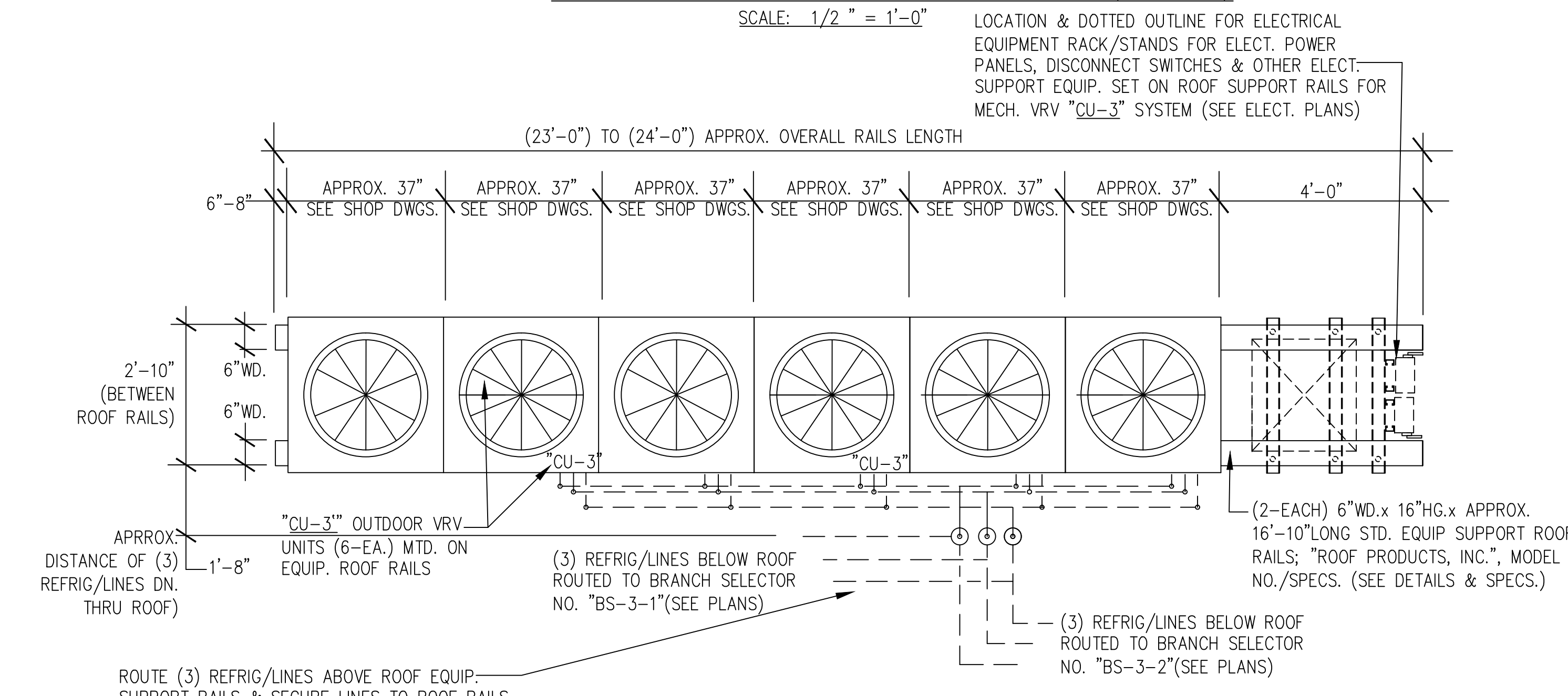
RUGBY - ENLARGED HVAC ROOF PLAN @ NEW "CU-3" VRV ZONE NO. 3 OUTDOOR UNITS (RUGBY) SCALE: 1/2" = 1'-0"
