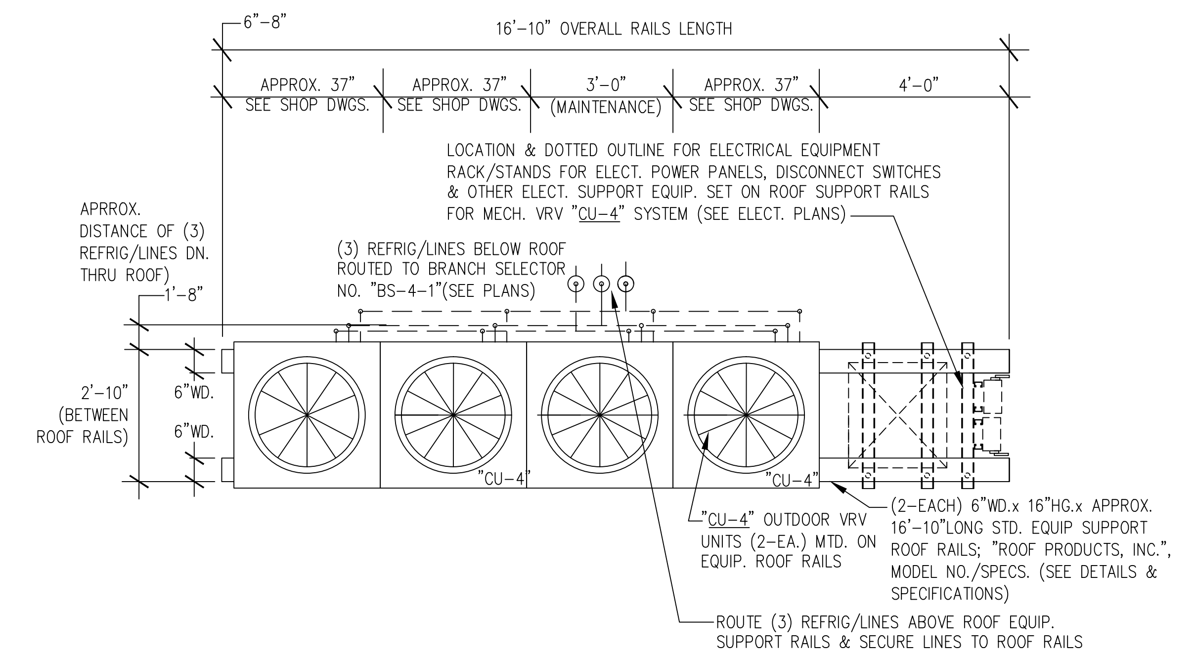
RUGBY - ENLARGED HVAC ROOF PLAN @ NEW "CU-4" VRV ZONE NO. 4 OUTDOOR UNITS (RUGBY) SCALE: 1/2" = 1'-0"
