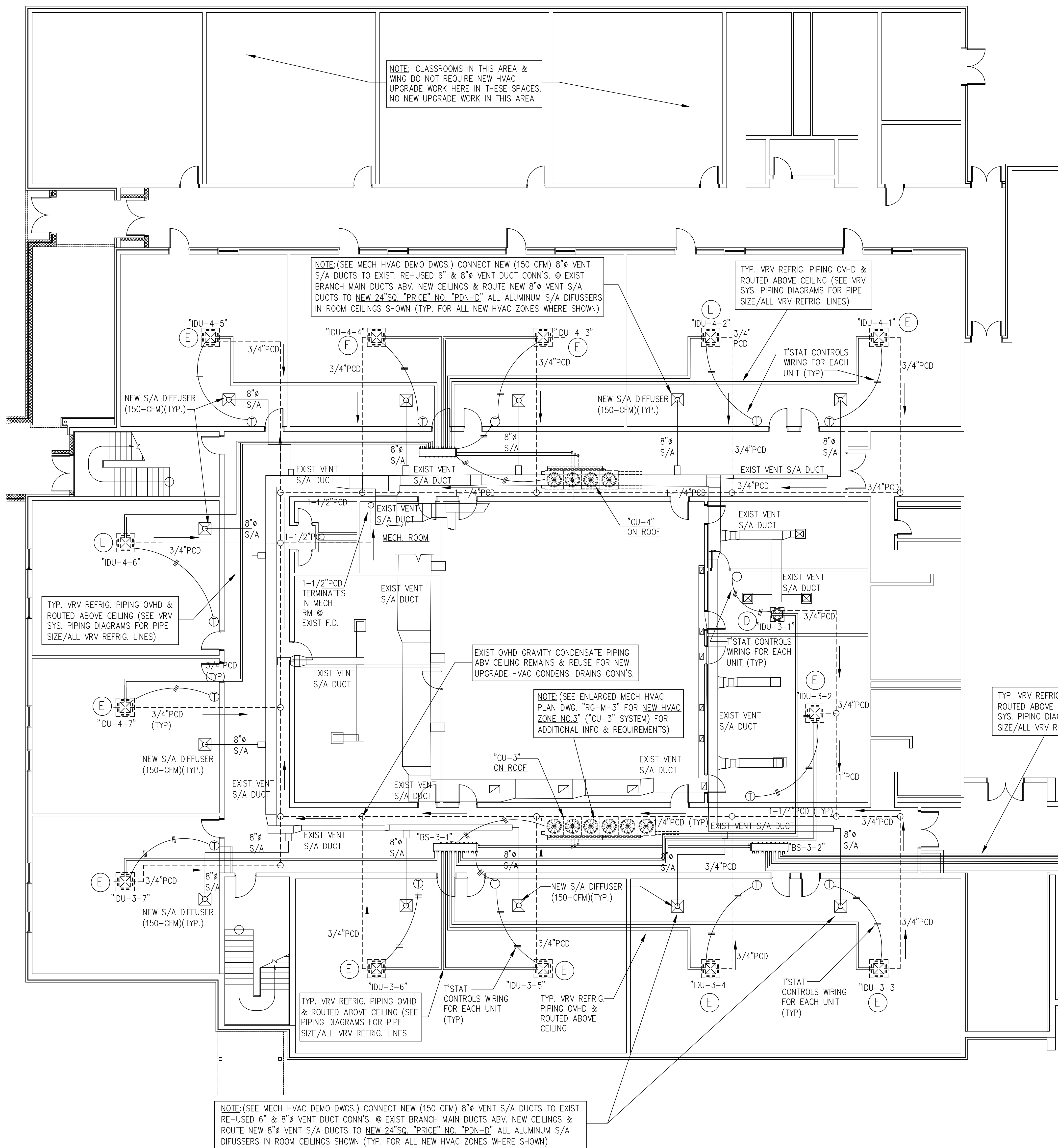
RUGBY HVAC UPGRADE NEW MECH. WORK - PART-A FLOOR PLAN @ EXIST. MAIN UPPER FLOOR (VRV ZONES 3 & 4) SCALE: 1/8"=1'-0" (EXIST REFERENCE PARTIAL FLOOR PLAN USED FOR NEW HVAC VRV SYSTEMS INFORMATION)
