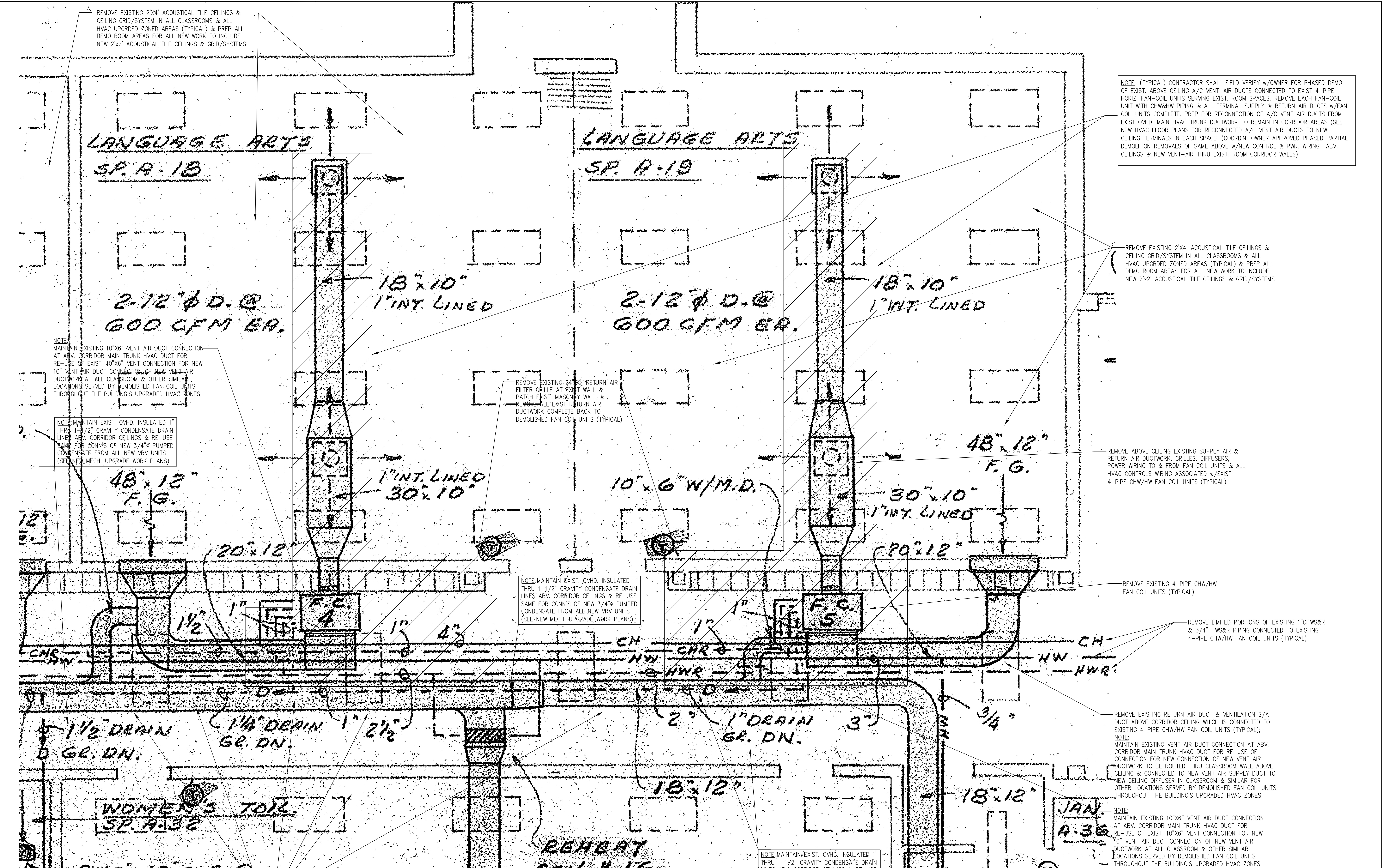
FLAT ROCK -HVAC UPGRADE DEMOLITION PART-A2 ENLARGED FLOOR PLAN @ TYPICAL CORRIDOR & CLASSROOM AREA @ EXIST. MAIN FLOOR SCALE: 1/2"=1'-0" (EXIST REFERENCE FLOOR PLAN USED FOR DEMOLITION INFORMATION ONLY)
