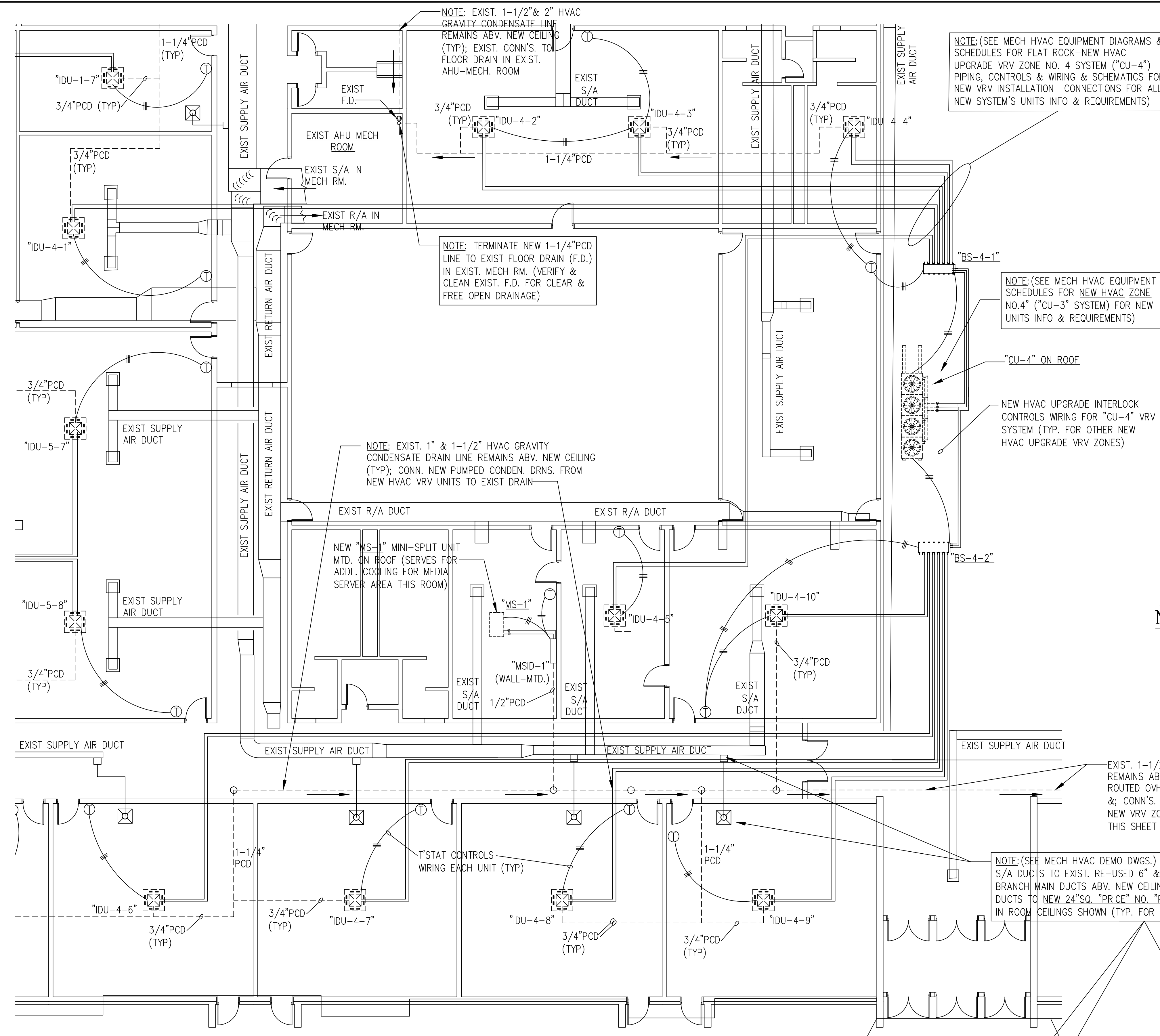
FLAT ROCK - NEW HVAC UPGRADE SYSTEMS - ENLARGED FLOOR PLAN @ NEW HVAC UPGRADE VRV ZONE NO. 4 SCALE: 1/8" = 1'-0"
