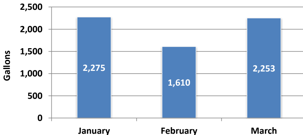
Henderson County CNG Fleet Fuel Consumption, Quarter 3 FY15 (January - March 2015) *
